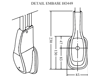
DETAIL EMBASE HO449
