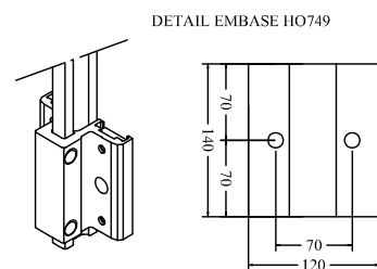
DETAIL EMBASE HO749
