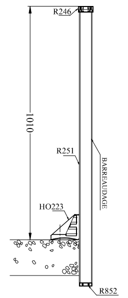
Version passant devant dalle
