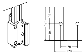
DETAIL EMBASE HO749
