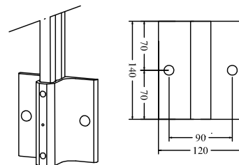
DETAIL EMBASE HO949
